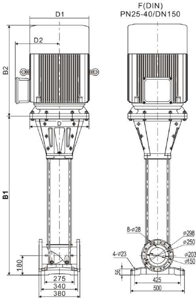
安装图/Installation sketch
